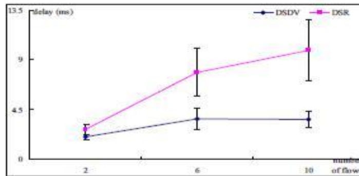
FIGURE1.3 Delay versus number of flows
