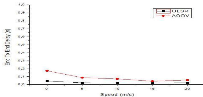
FIGURE.1.4 Delay versus Speed Graph
