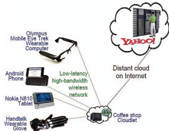
Fig. 6: Concept and Infrastructure of Cloudlet [23]
