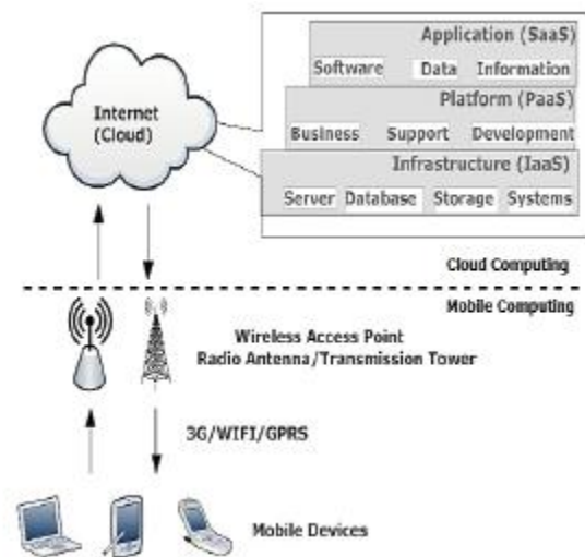
Fig. 3: Architecture of Mobile Cloud Computing
