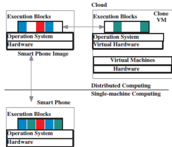
Fig. 4: CloneCloud System Architecture
