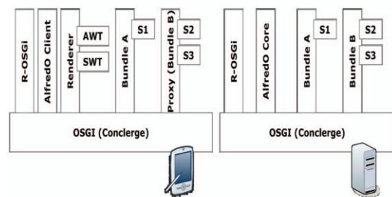
Fig. 5: AlfredO Architecture
