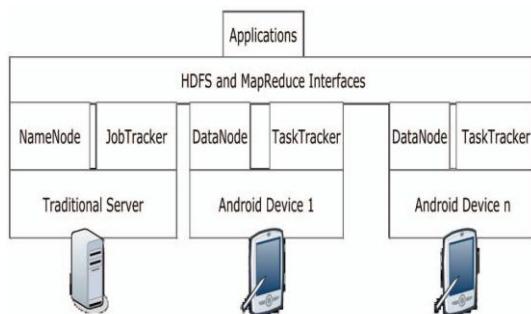
Fig. 7: Hyrax Infrastructure
